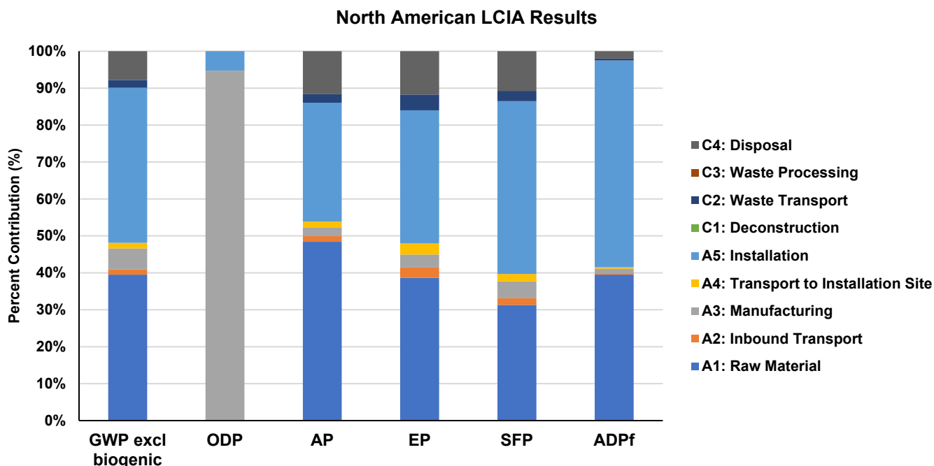
Figure 6: Contribution analysis of North American LCIA Results
