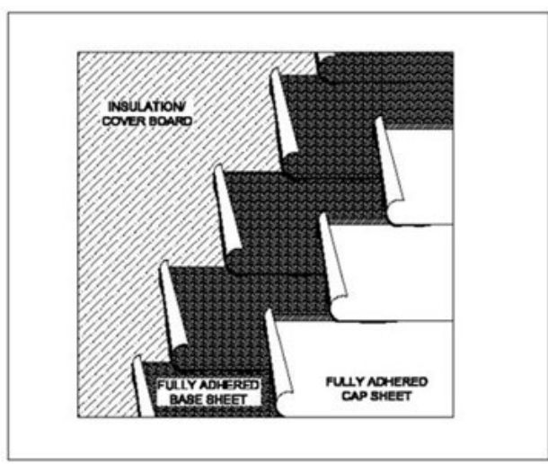
Figure 3: APP modified bitumen roof membrane system installation details
