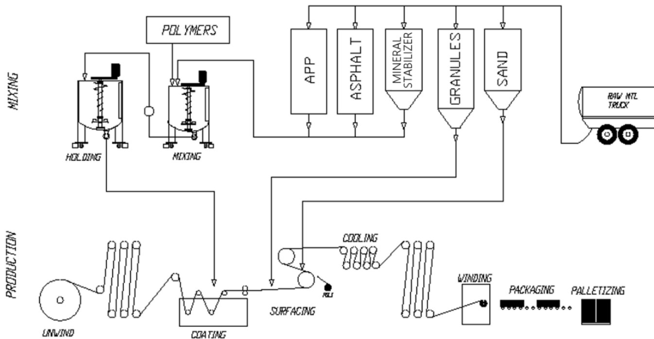
Figure 2: Modified bitumen sheet process diagram for APP base sheet and cap sheet
