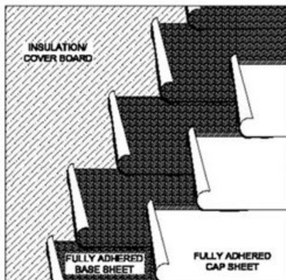
Figure 3: APP modified bitumen roof membrane system installation details
