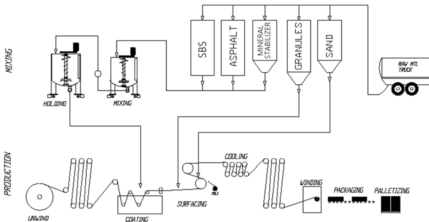
Figure 2: Modified bitumen sheet process diagram
