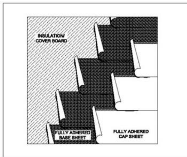
Figure 3: APP modified bitumen roof membrane system installation details
