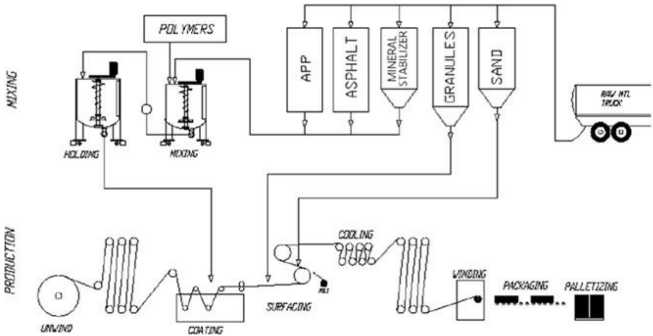
Figure 2: Modified bitumen sheet process diagram for APP cap sheet
