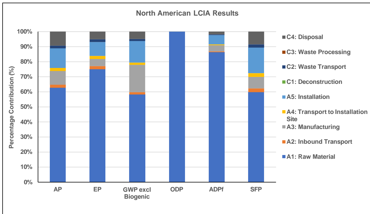
Figure 5: Contribution analysis of North American LCIA results
