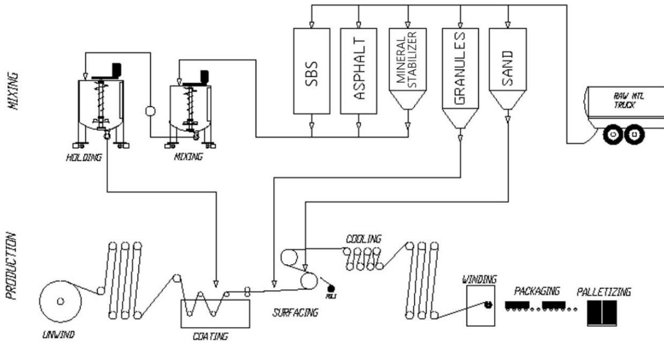
Figure 3: Modified bitumen sheet process diagram for SBS base sheet
