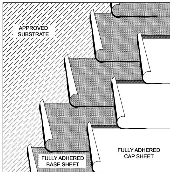
Figure 4: Hybrid modified bitumen roof membrane system installation details
