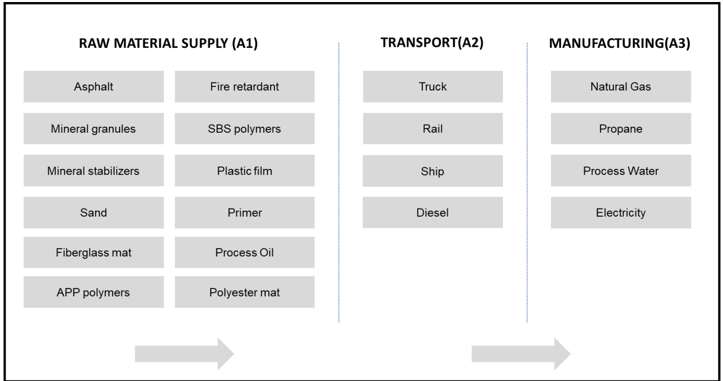
Figure 1: Production process overview
